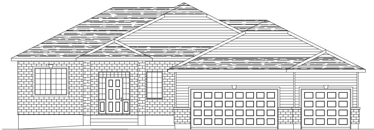
FRONT ELEVATION
